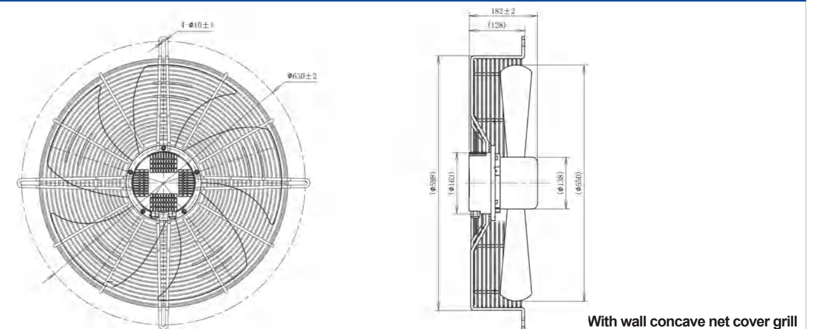
LWAE3G550TS-5MEW-03(Suction)
