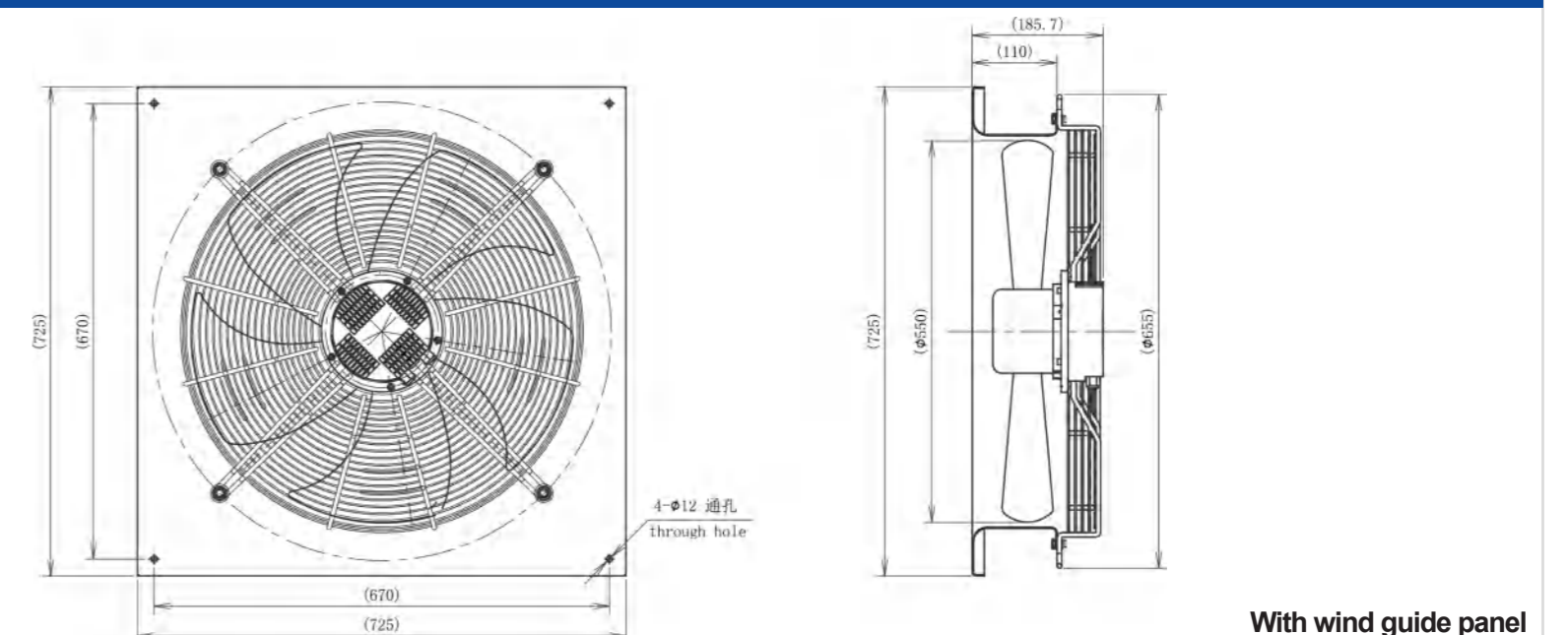
LWAE3G550TS-5MGW-05(Suction)
