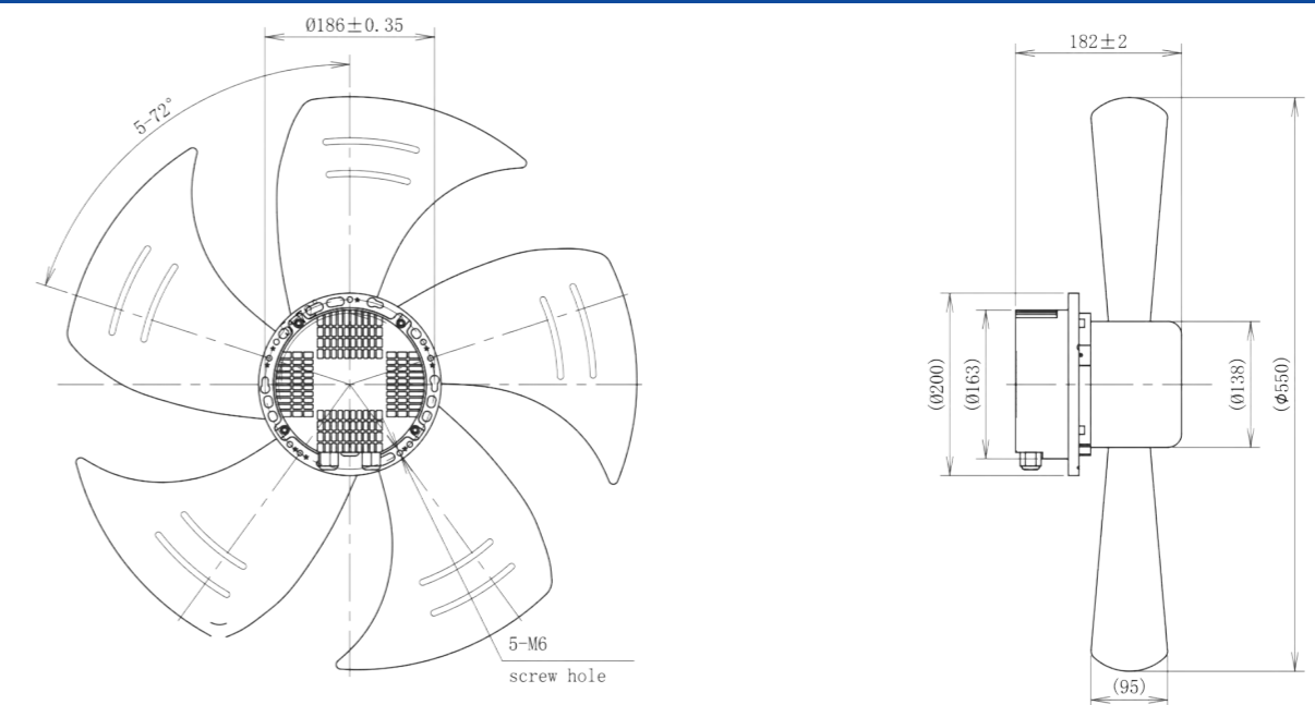
LWAE3G550TS-5MNW-01(Suction)
