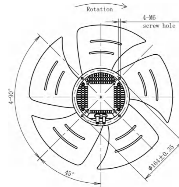
LWAE3G450SS-5MNW-01(Suction)
