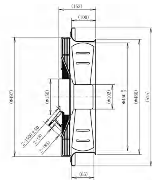
LWAE3G450ST-5MGW-06(Blowing)
