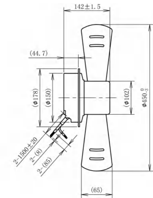
LWAE3G450ST-5MEW-04(Blowing)
