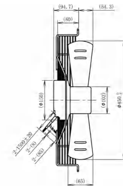
LWAE3G450ST-5MGW-06(Blowing)
