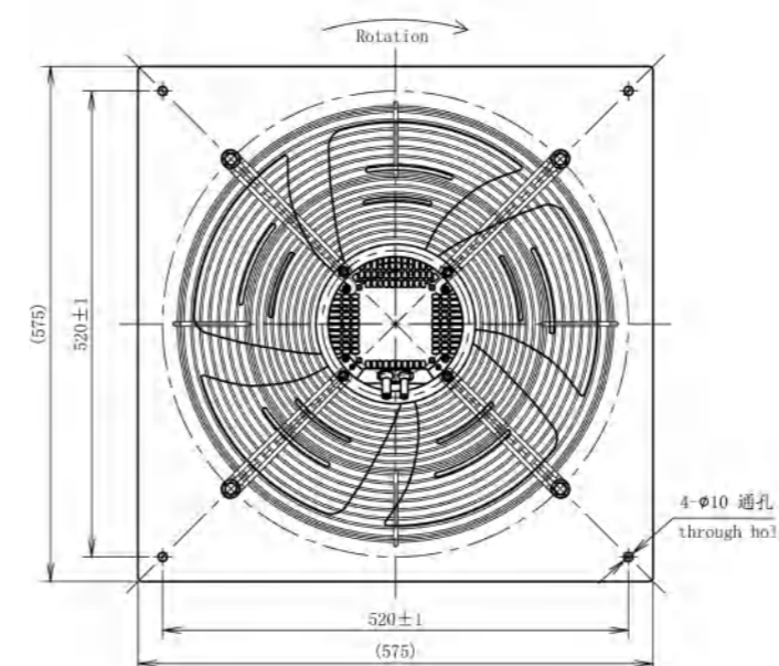
LWAE3G450SS-5MGW-05(Suction)
