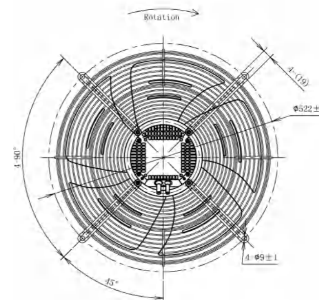
LWAE3G450SS-5MGW-05(Suction)
